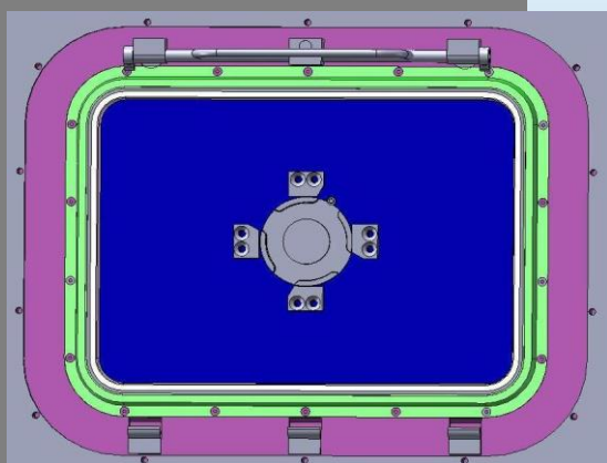
Porte STERIPASS® 290 – brevet international
